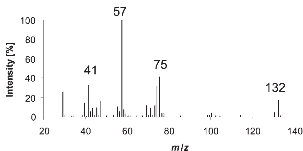
Figure 7. Mass spectrum (MS-EI) of odorant 15 (4-mercapto-3-hexanone).
