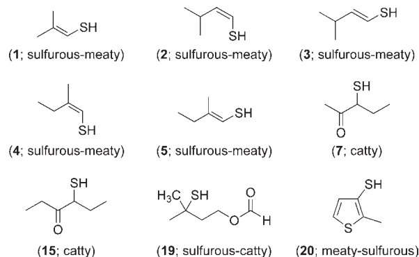
Figure 8. Chemical structures of the compounds identified for the first time in roasted sesame or in foods ( 1–5 , 15 ), respectively.
