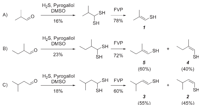
Figure 3. Synthetic approach used in the preparation of (A) 2-methyl-1-propene-1-thiol ( 1 ), (B) ( E )-2-methyl-1-butene-1-thiol ( 5 ) and ( Z )-2-methyl-1-butene-1-thiol ( 4 ), and (C) ( E )-3-methyl-1-butene-1-thiol ( 3 ) and ( Z )-3-methyl-1-butene-1-thiol ( 2 ).
