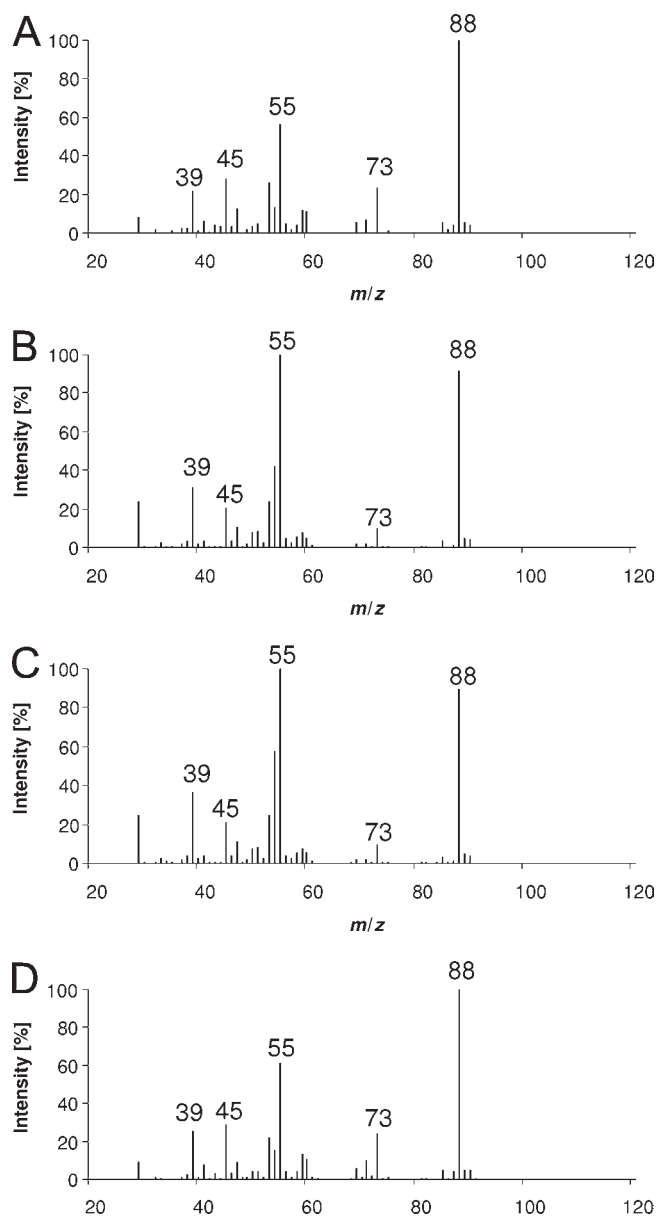
Figure 5. Mass spectra (MS-EI) of odorant 1 (A), ( E )-2-butene-1-thiol (B), ( Z )-2-butene-1-thiol (C), and 2-methyl-1-propene-1-thiol (D; I ).
