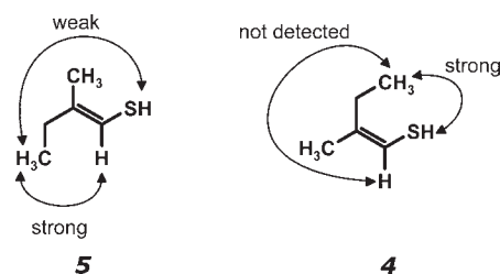
Figure 4. NOE observed for synthesized ( E )-2-methyl-1-butene-1-thiol ( 5 ) and ( Z )-2-methyl-1-butene-1-thiol ( 4 ).
