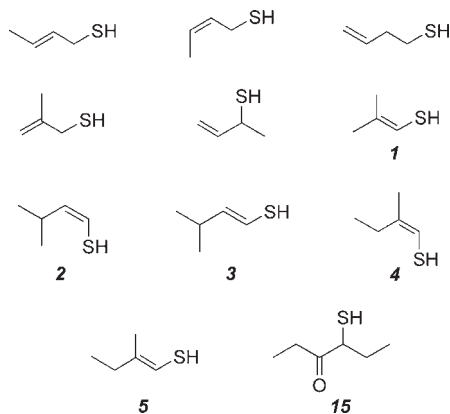
Figure 1. Structures of the 11 thiols prepared by synthesis. Only compounds also identified in sesame seeds are numbered. Numbers of synthesized reference compounds are italicized to differentiate them from the sesame odorants.
