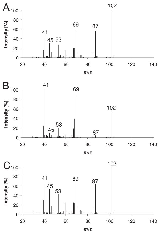
Figure 6. Mass spectra (MS-EI) of odorant 5 (A), 3-methyl-2-butene-1-thiol (B), and ( E )-2-methyl-1-butene-1-thiol (C; 5 ).
